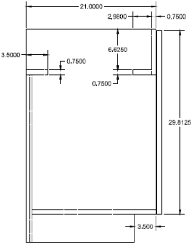
SIDE VIEW
